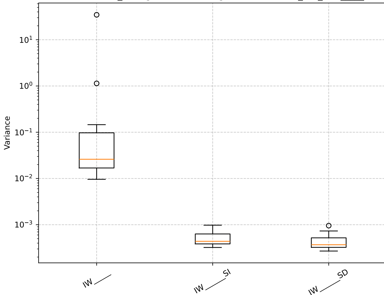
Q=1.14, len_rolling=100: Shrinkage Box Plot - min_var_, IW_____
