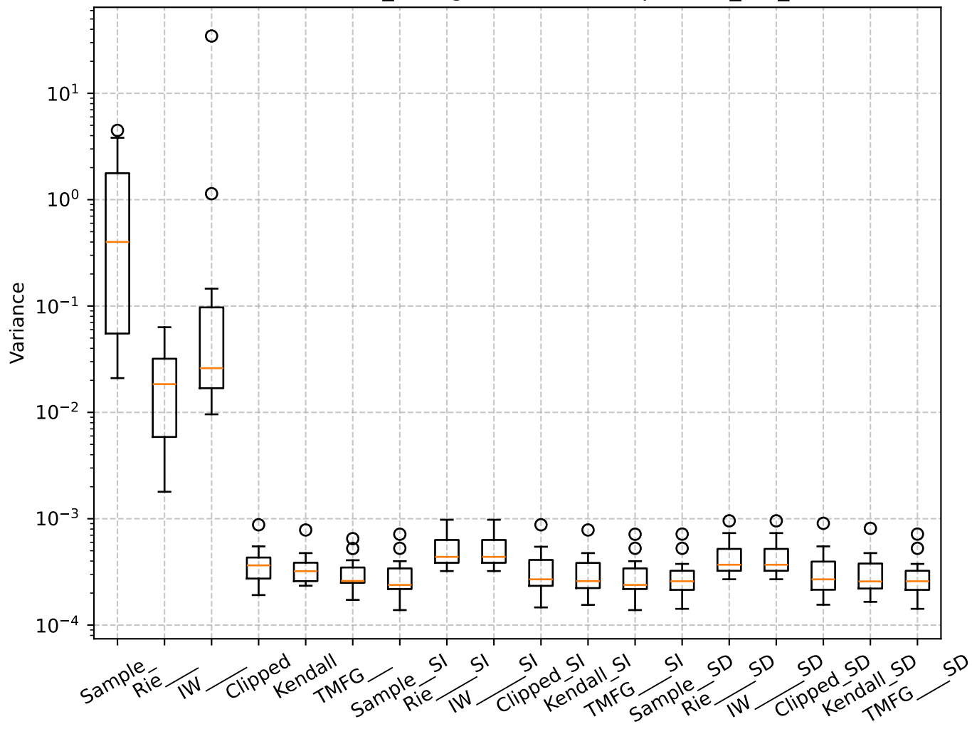
Q=1.14, len_rolling=100: Box Plot per min_var_
