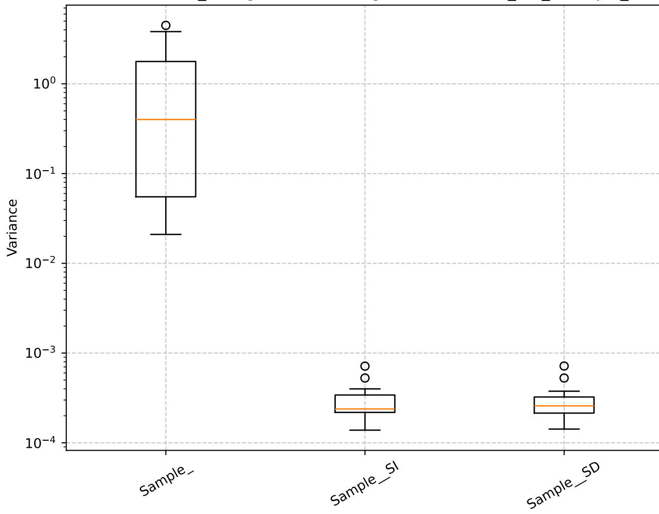
Q=1.14, len_rolling=100: Shrinkage Box Plot - min_var_, Sample_
