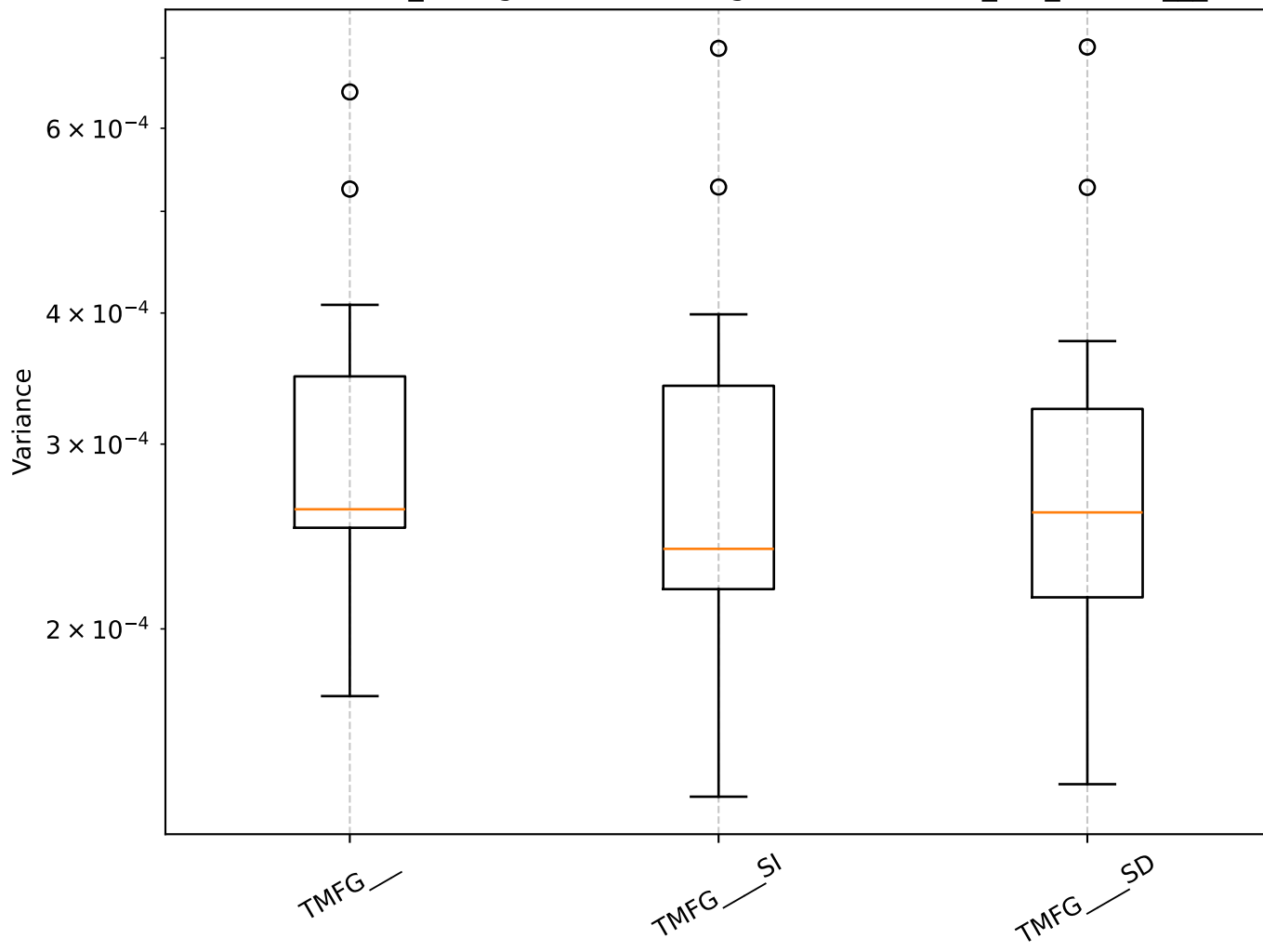
Q=1.14, len_rolling=100: Shrinkage Box Plot - min_var_, TMFG__
