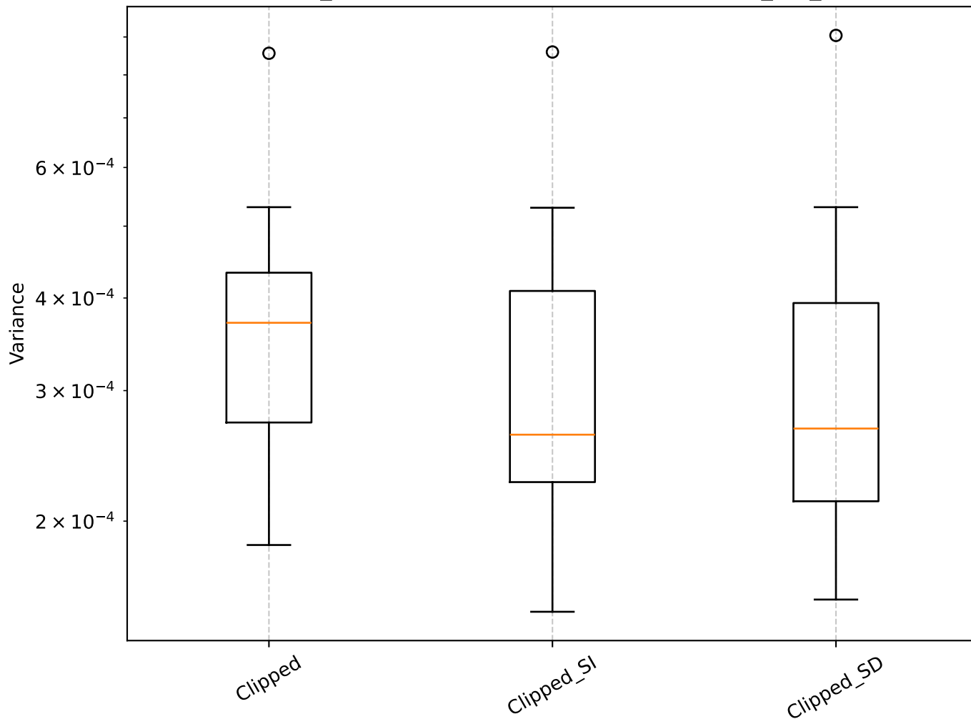
Q=1.18, len_rolling=100: Shrinkage Box Plot - min_var_, Clipped
