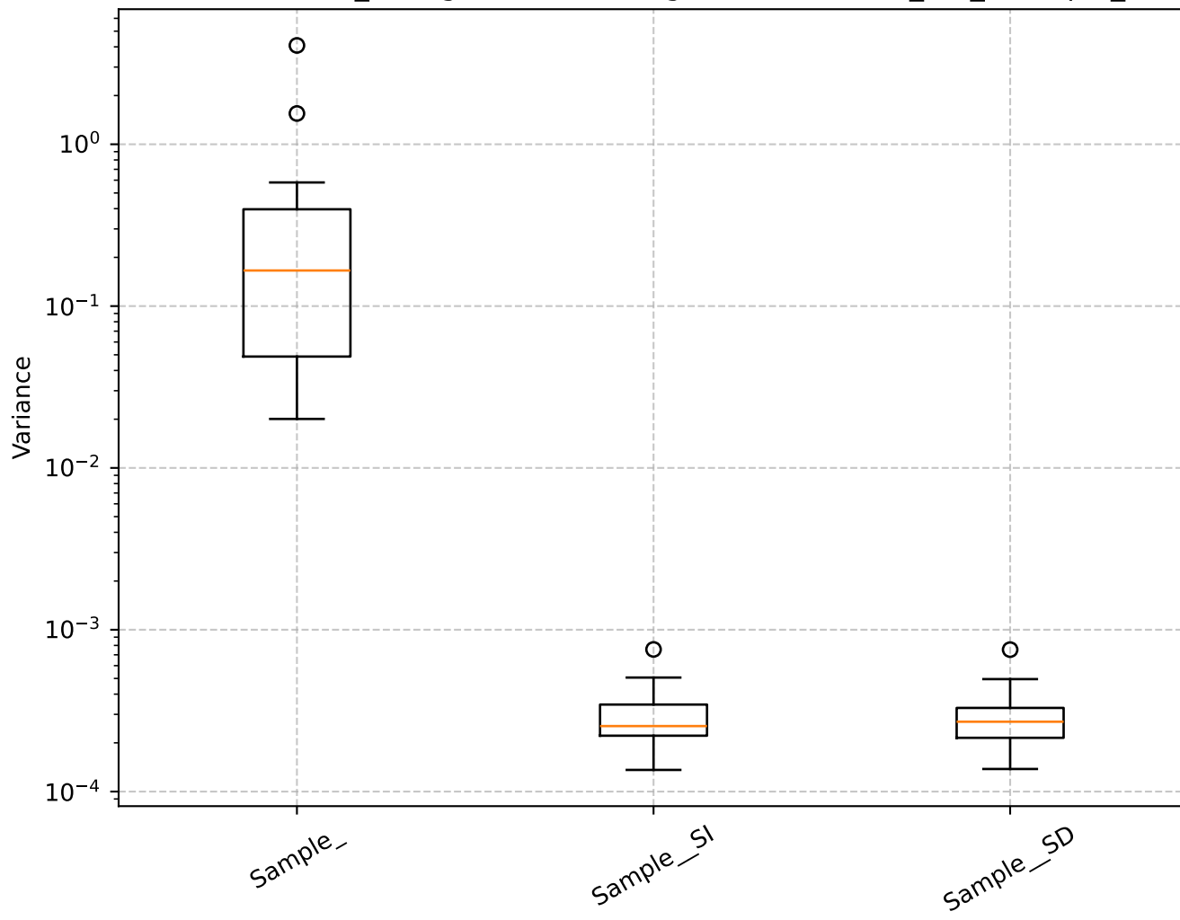
Q=1.33, len_rolling=100: Shrinkage Box Plot - min_var_, Sample_
