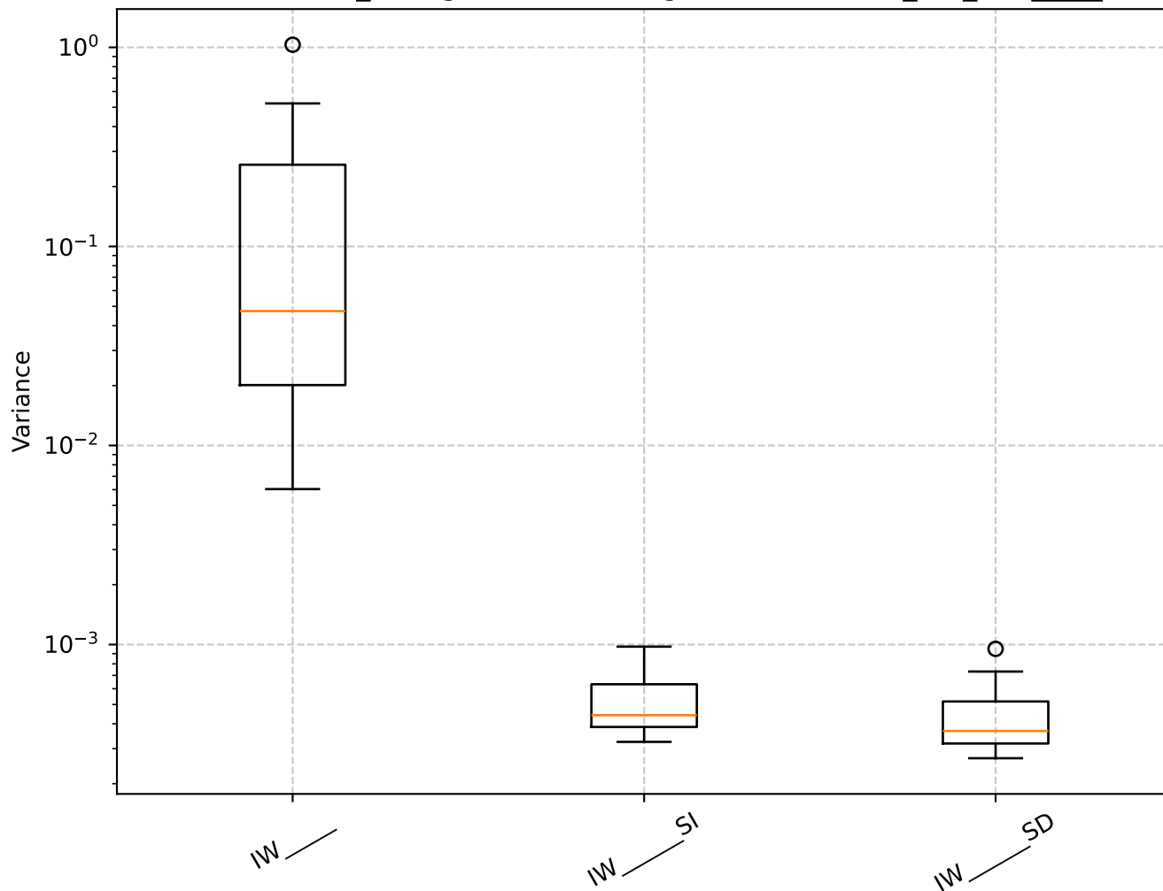
Q=1.38, len_rolling=100: Shrinkage Box Plot - min_var_, IW_____
