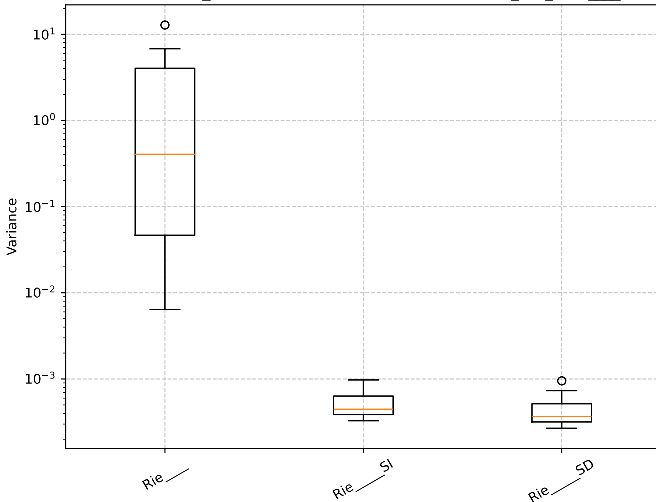
Q=1.54, len_rolling=100: Shrinkage Box Plot - min_var_, Rie_
