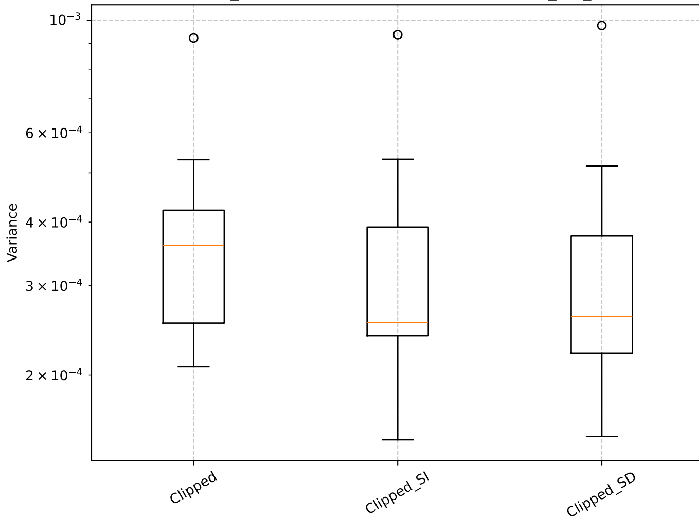
Q=1.60, len_rolling=100: Shrinkage Box Plot - min_var_, Clipped
