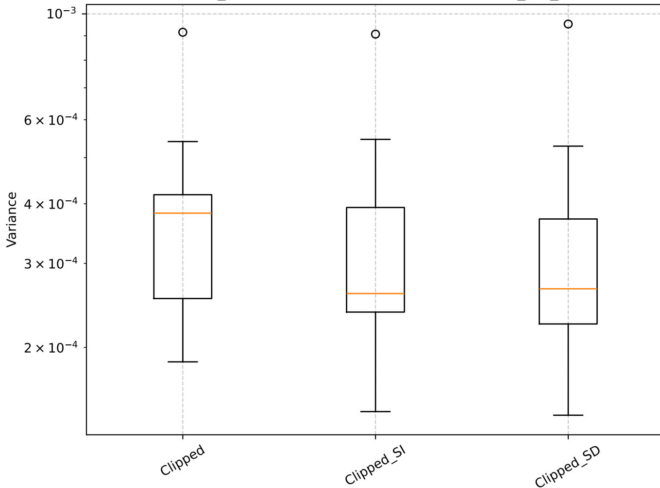
Q=1.75, len_rolling=100: Shrinkage Box Plot - min_var_, Clipped
