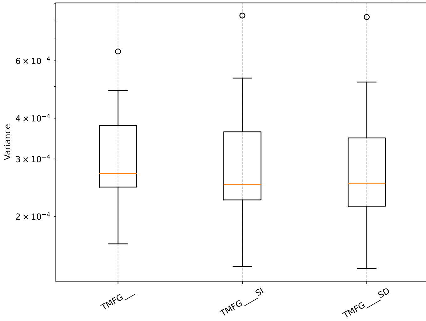
Q=1.83, len_rolling=100: Shrinkage Box Plot - min_var_, TMFG__
