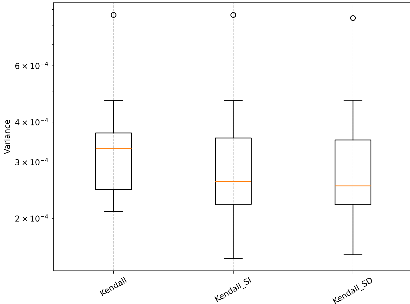
Q=1.90, len_rolling=100: Shrinkage Box Plot - min_var_, Kendall
