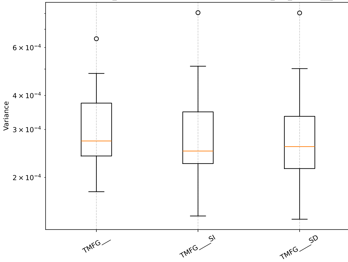
Q=1.90, len_rolling=100: Shrinkage Box Plot - min_var_, TMFG__
