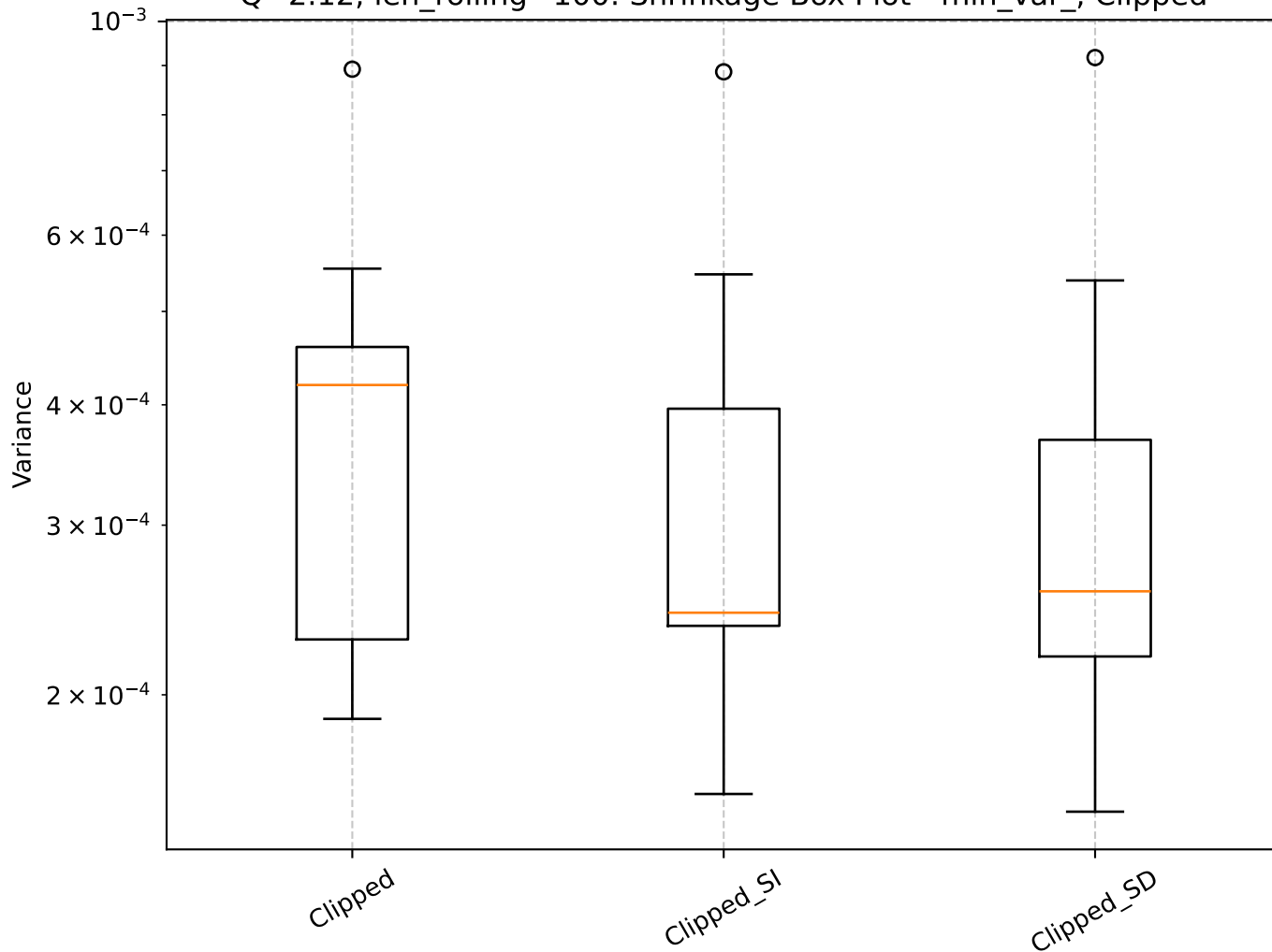
Q=2.12, len_rolling=100: Shrinkage Box Plot - min_var_, Clipped
