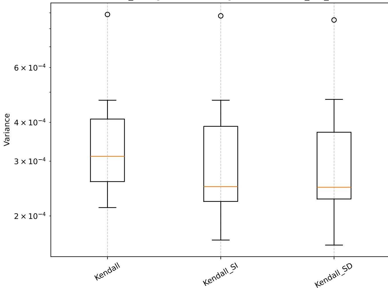
Q=2.12, len_rolling=100: Shrinkage Box Plot - min_var_, Kendall
