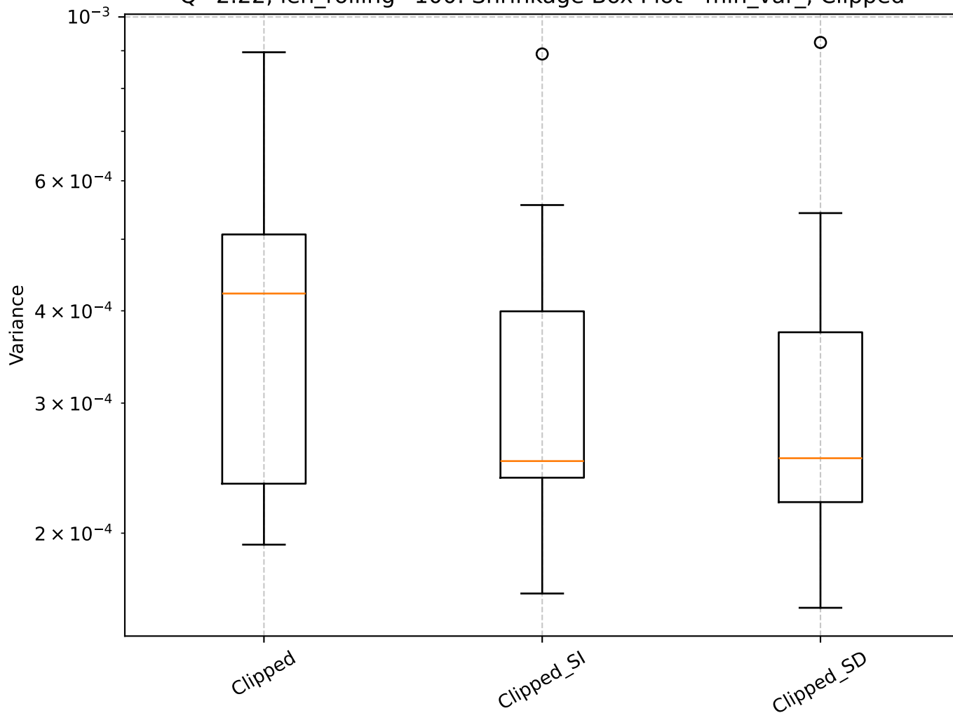
Q=2.22, len_rolling=100: Shrinkage Box Plot - min_var_, Clipped
