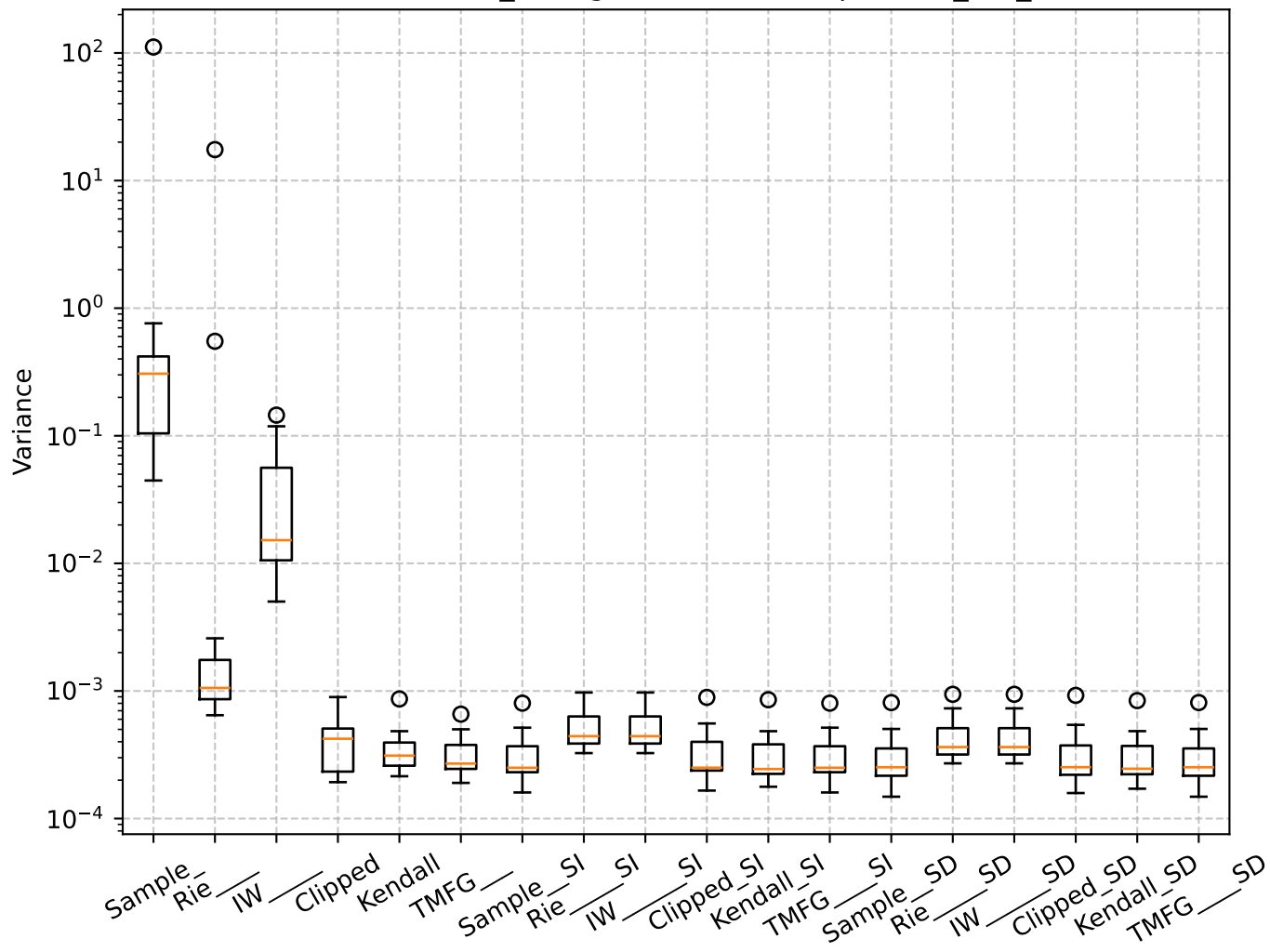
Q=2.22, len_rolling=100: Box Plot per min_var
