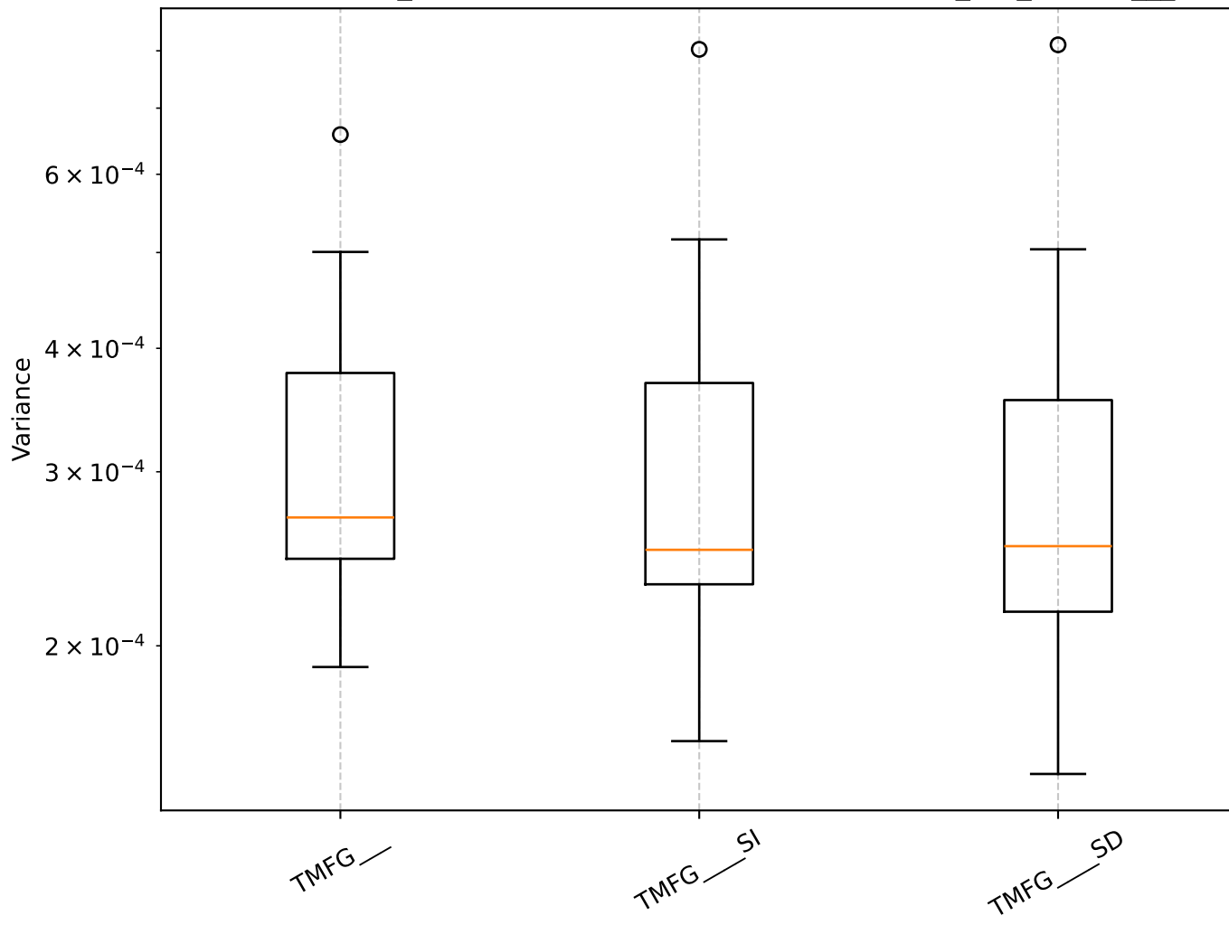
Q=2.22, len_rolling=100: Shrinkage Box Plot - min_var_, TMFG__
