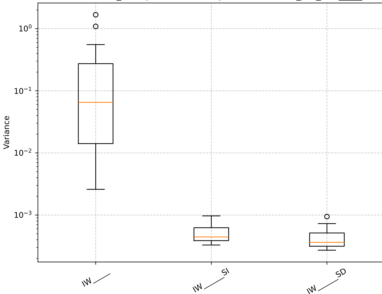
Q=2.68, len_rolling=100: Shrinkage Box Plot - min_var_, IW_____
