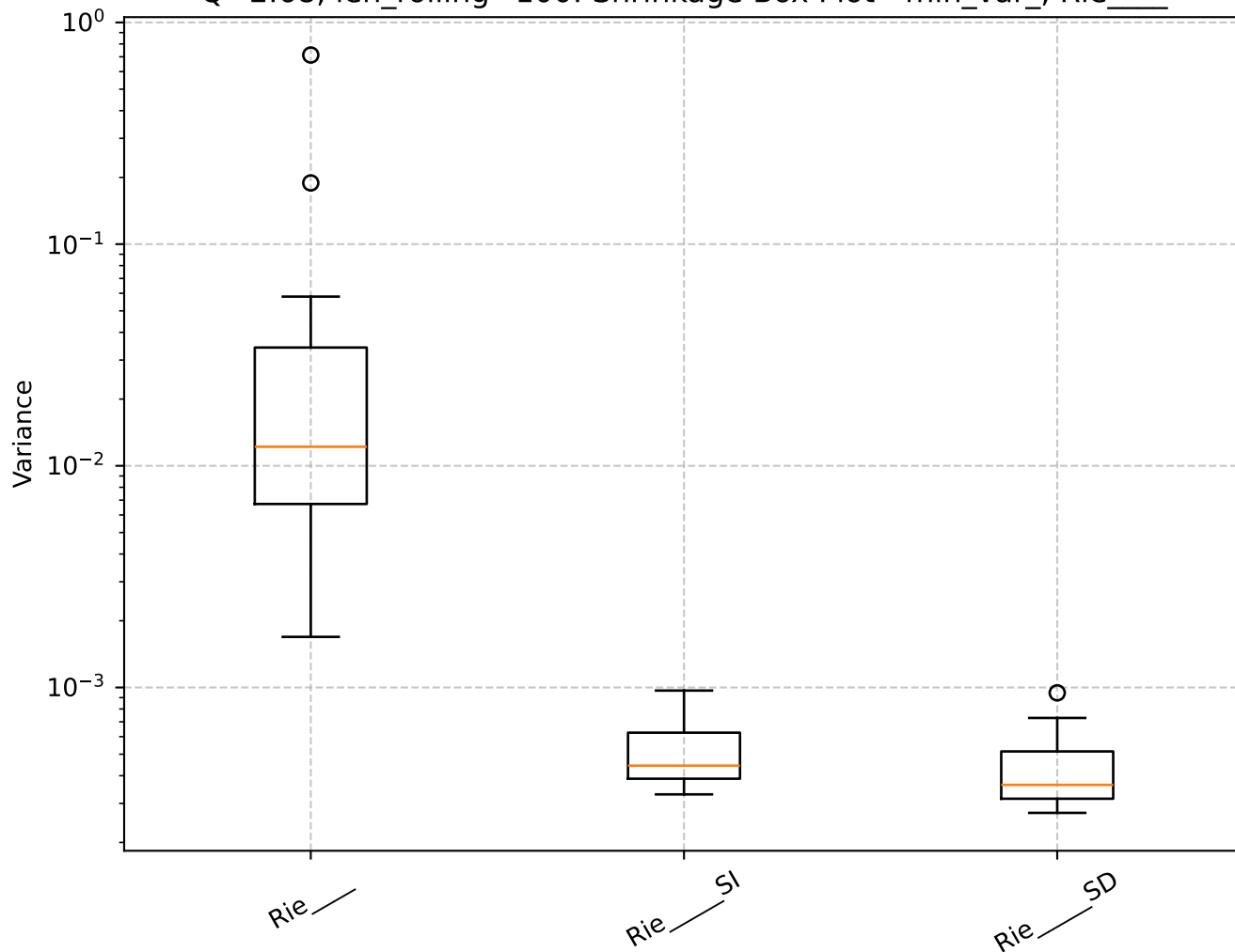
Q=2.68, len_rolling=100: Shrinkage Box Plot - min_var_, Rie____
