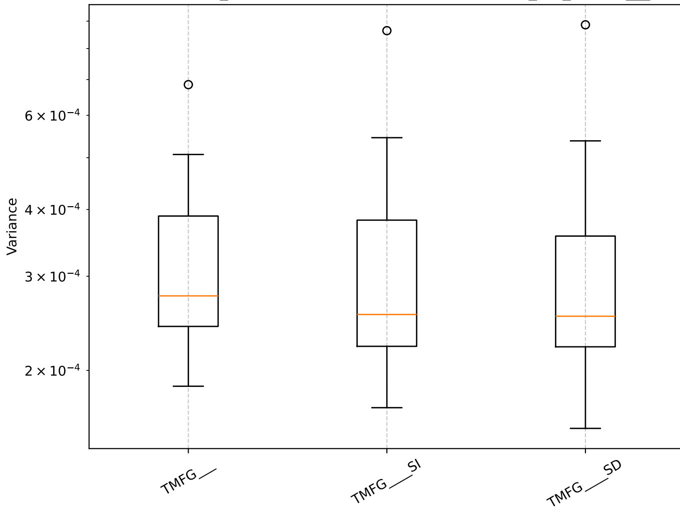
Q=3.10, len_rolling=100: Shrinkage Box Plot - min_var_, TMFG__
