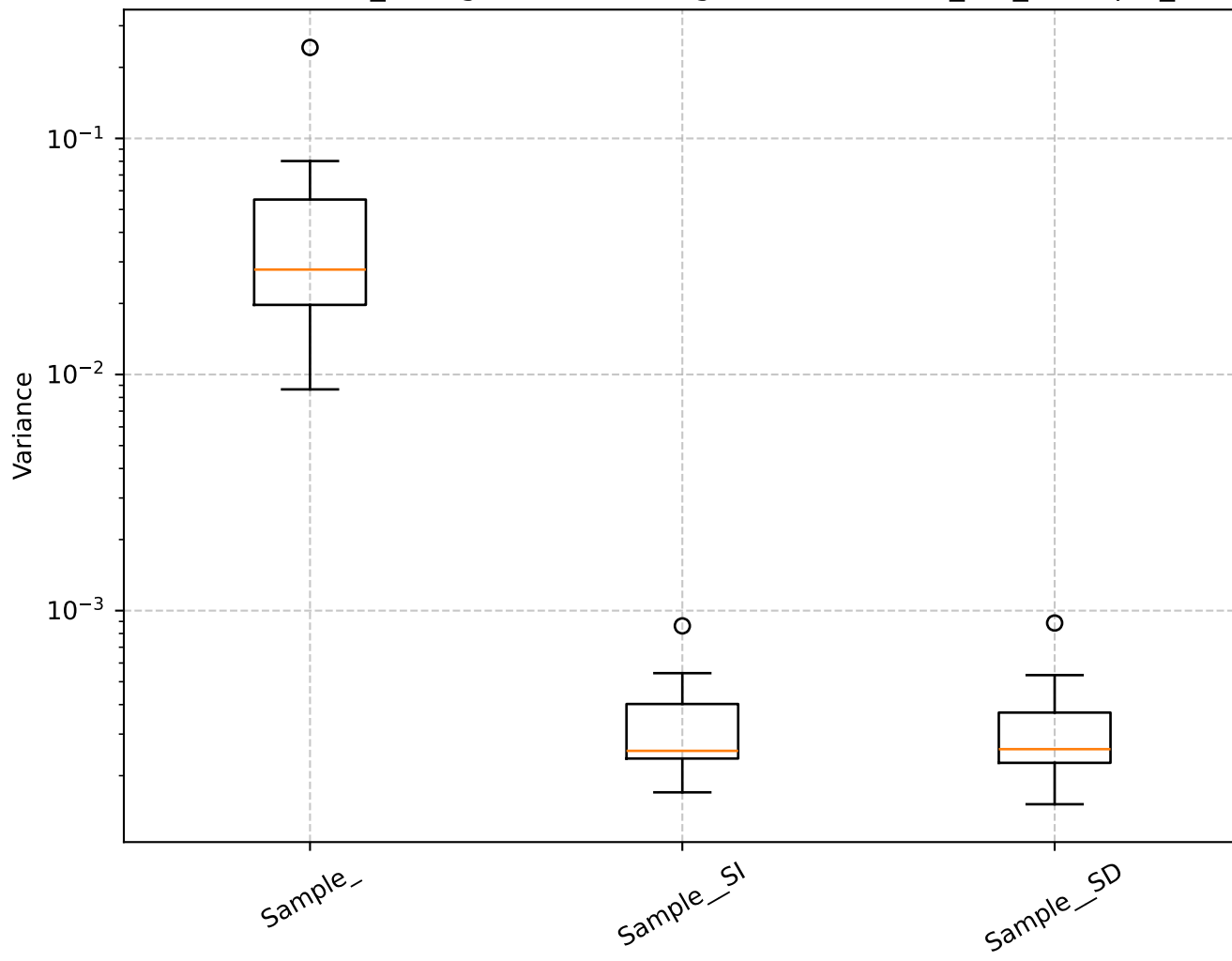
Q=3.33, len_rolling=100: Shrinkage Box Plot - min_var_, Sample_
