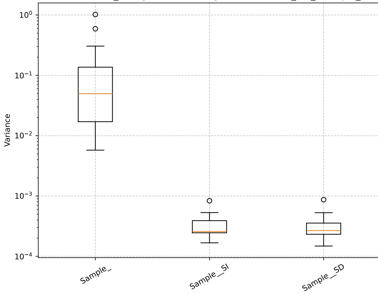
Q=3.67, len_rolling=100: Shrinkage Box Plot - min_var_, Sample_
