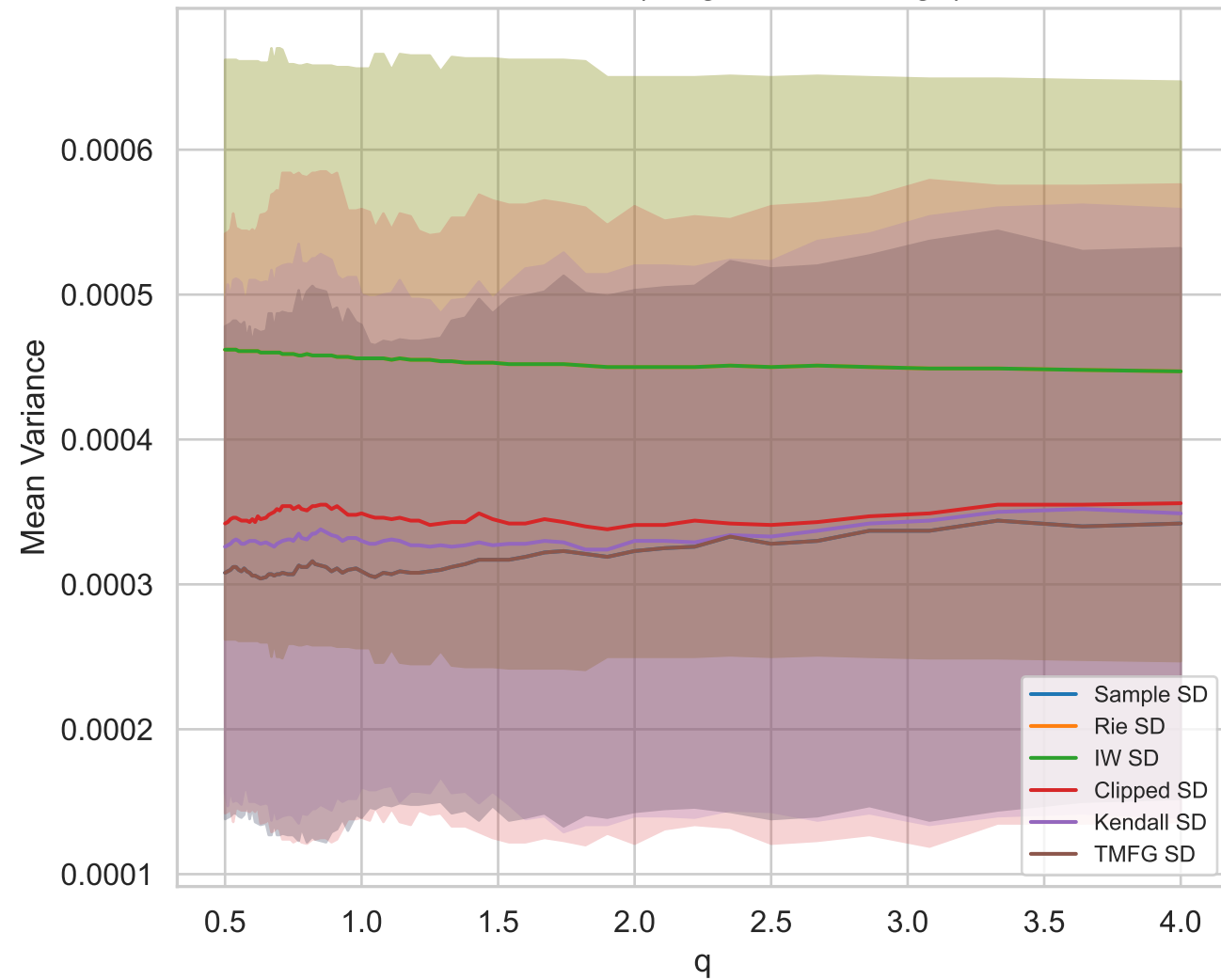
All Methods (Diagonal Shrinkage)
