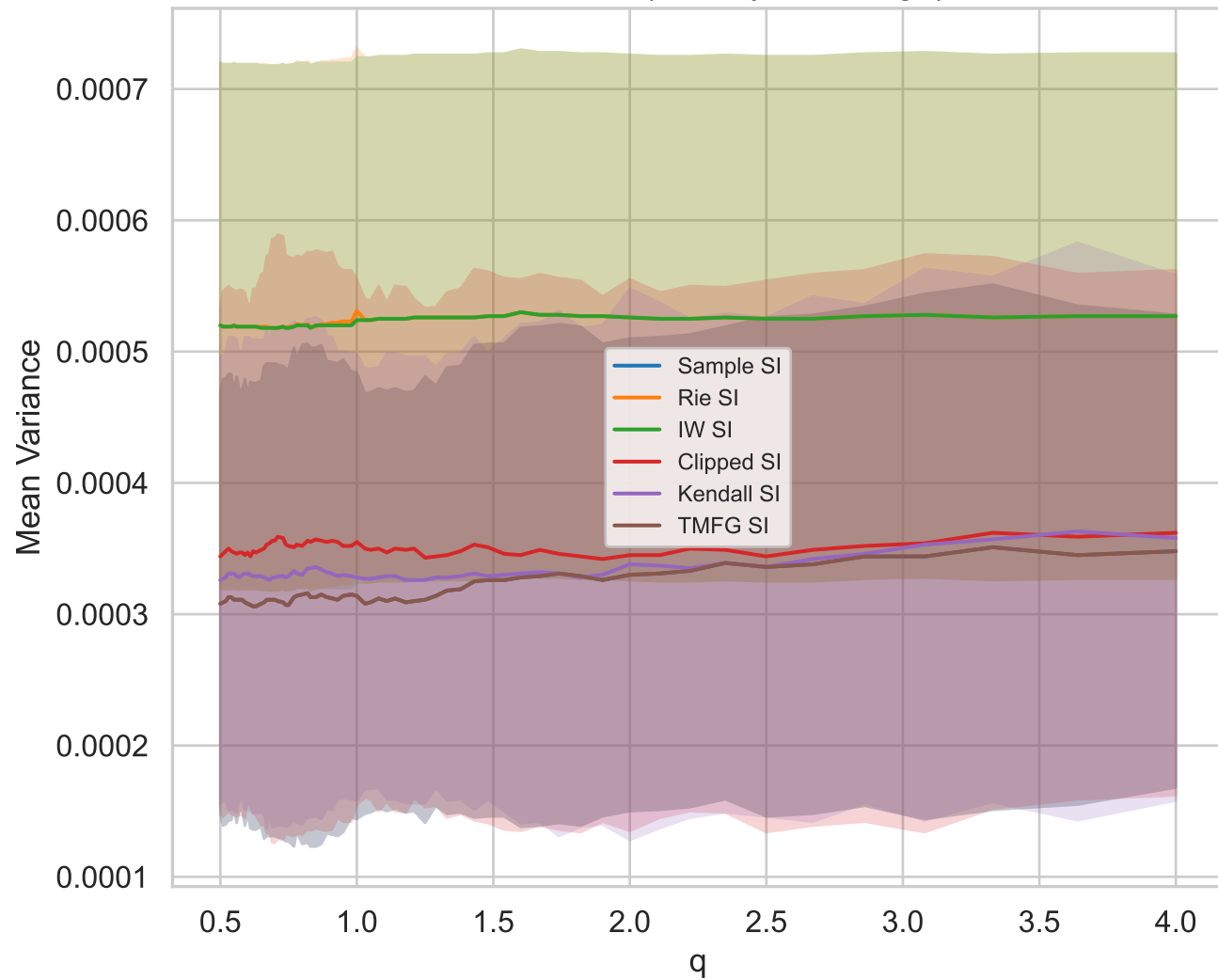
All Methods (Identity Shrinkage)
