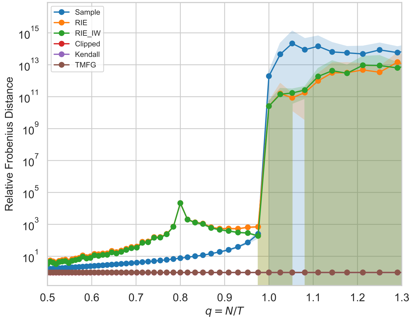
All Methods (Zoomed in q )
