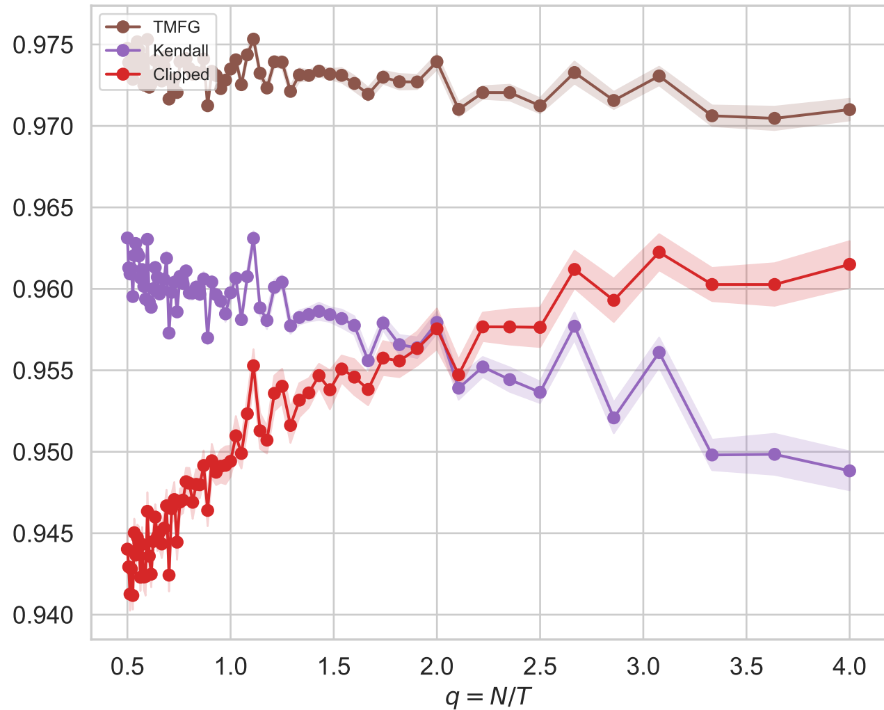
Robust Methods (Full Range)
