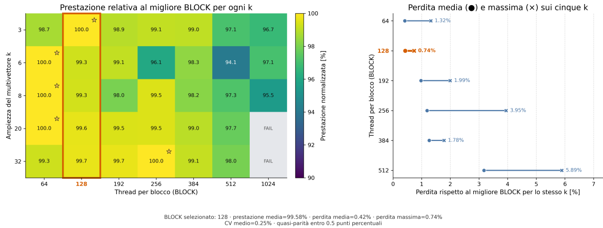
(a) cuda_warp, X column-major.
