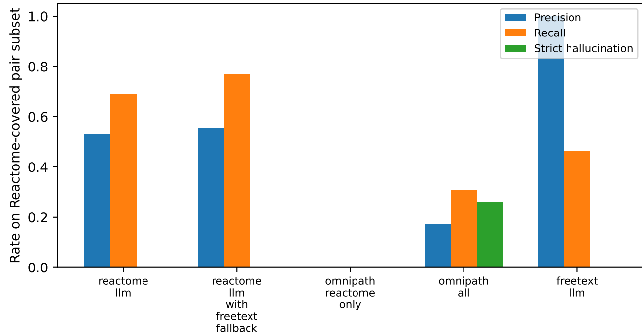
Sachs: constraint quality conditional on Reactome evidence
