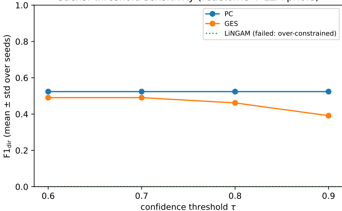
Sachs: threshold sensitivity (reactome + LLM priors)
