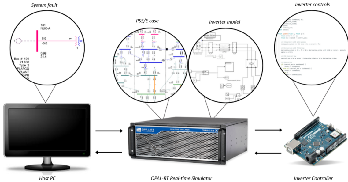
Figure 1: HIL System Overview
