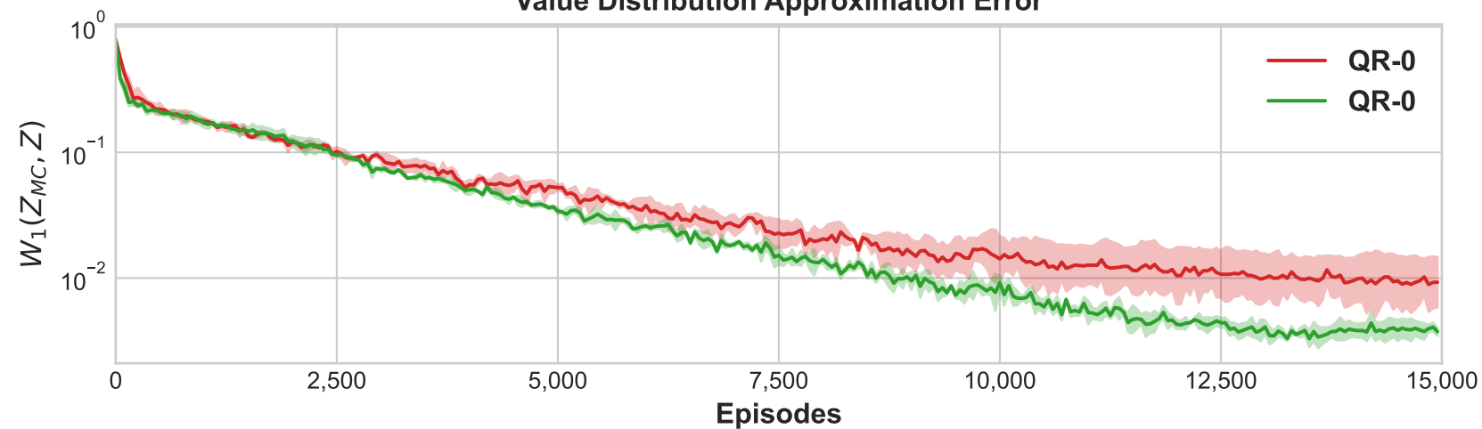
Value Distribution Approximation Error
