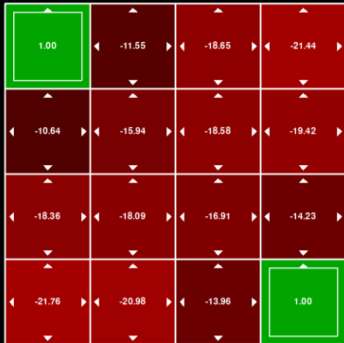
MC evaluation of SmallGridworld-v0 using first-visit
