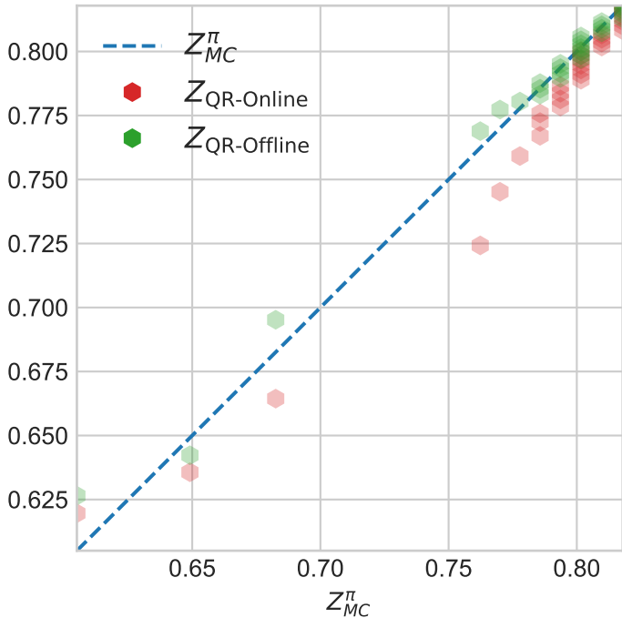
Estimated Quantiles
