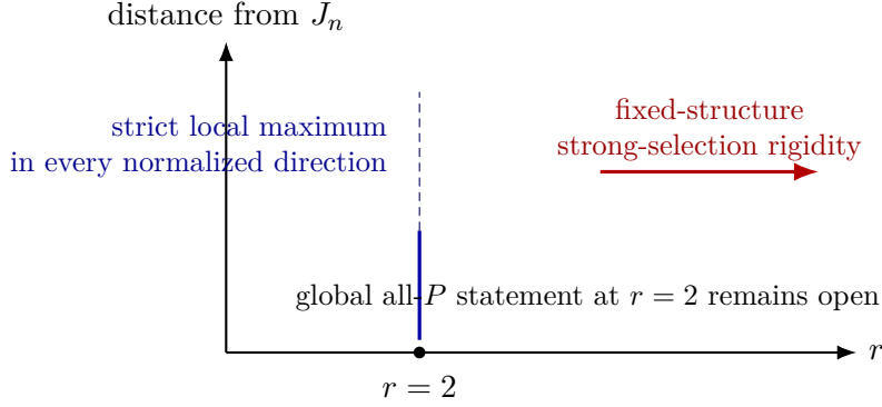
Figure 1: The two proved axes of the same complete-kernel deficit. The fitness-two theorem is local in the full normalized structure space and valid for every population size; the strong-selection theorem is global in fixed finite structure and asymptotic in fitness.
