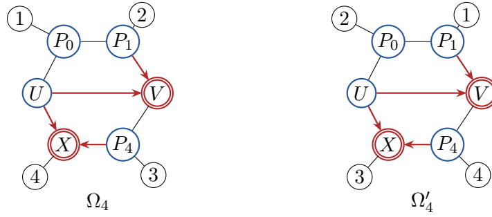
Figure 6: The triangle-free Omega sharpness pair. Both mixed graphs have cycle lengths 4, 4, 6 and the same arrowhead pattern; the labelled pendant attachments are (1, 2, 3, 4) on the left and (2, 1, 4, 3) on the right. Each graph has seven admissible rootings, exactly two of which are tree-child. Up to reflection, both have quarnet type (2c) in the taxonomy of Englander et al. [6, Figure 5].
