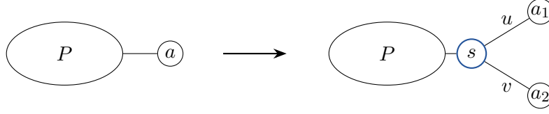
Figure 5: Identical cherry substitution at corresponding leaves. In Fourier coordinates the two new arms multiply the old port tensor, and positive ratios recover u , v , and the original tensor analytically. Each added leaf therefore contributes exactly two dimensions while leaving every nontrivial blob unchanged.
