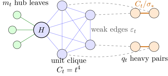
Figure 1: Schematic of the dilute hybrid. Dashed lines show representative satellite–clique edges, all of weight \varepsilon_t ; every satellite vertex is adjacent to every clique vertex.
