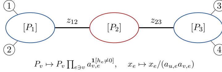
Figure 3: Bridge-tree peeling recovers a projective local tensor orbit [P_v] at each retained component and normalized effective bridge scales z_e . The original physical bridge multiplier is not an intrinsic coordinate; the exact fiber is the full incidence-scaling orbit intersected with the positive JC domain.
