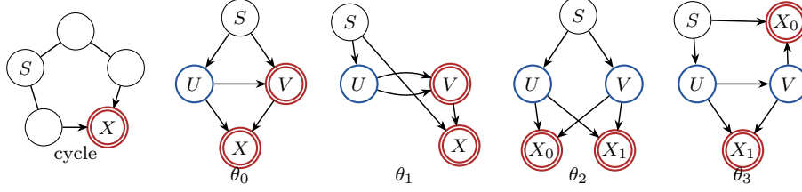
Figure 2: The primitive directed skeletons used by the local theorem: one cycle and four theta orientations. Parallel skeleton sides, visible in \theta_1 , must be subdivided by an occupied port before the fixed mixed graph is admitted as simple. Minimum strong repairs and arbitrary port subdivisions are added to these skeletons by the structural theorem.
