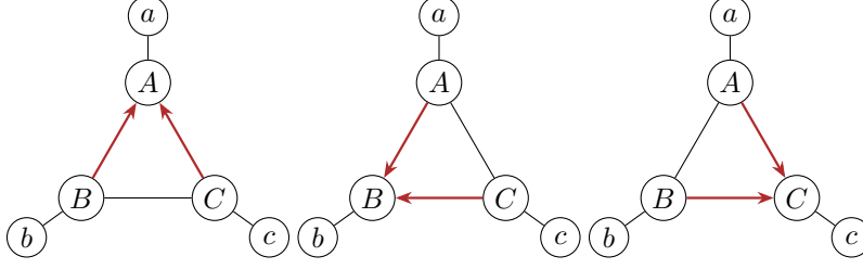
Figure 4: Ordinary triangle redirection T . The labelled underlying graph and all external attachments are fixed; only the reticulation vertex and the two incoming arrowheads inside the triangle change. The three local JC models share a regular full-dimensional germ, not necessarily their entire open stochastic images.
