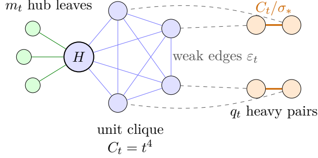
Figure 1: Schematic of the dilute hybrid. Dashed lines show representative satellite–clique edges, all of weight \varepsilon_t ; every satellite vertex is adjacent to every clique vertex.
