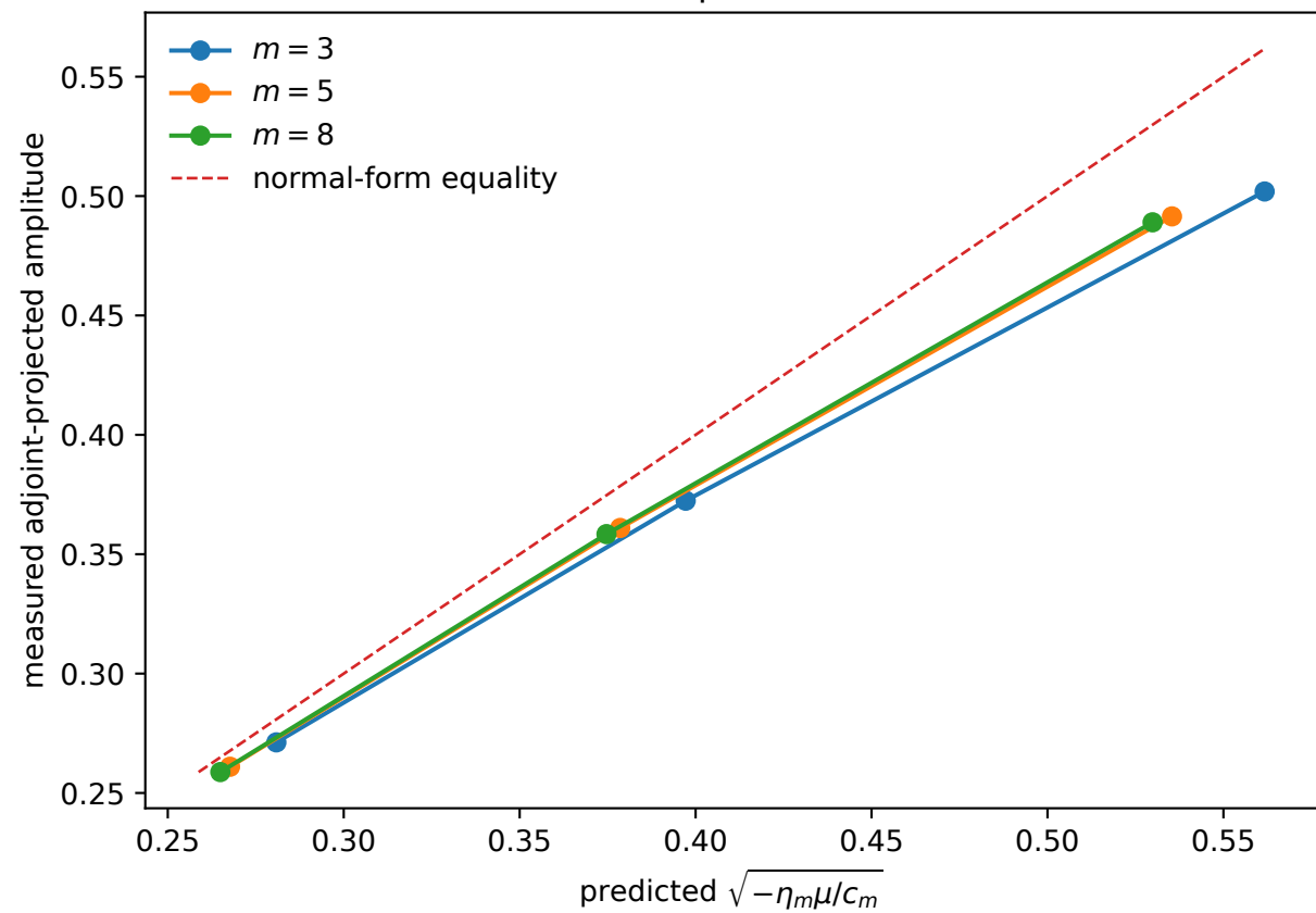
First-mode amplitude near onset
