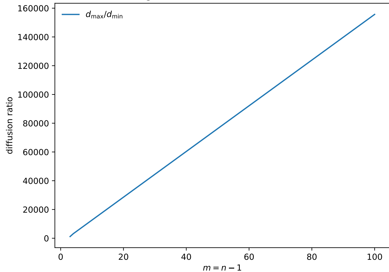
Linear growth of the exact diffusion contrast
