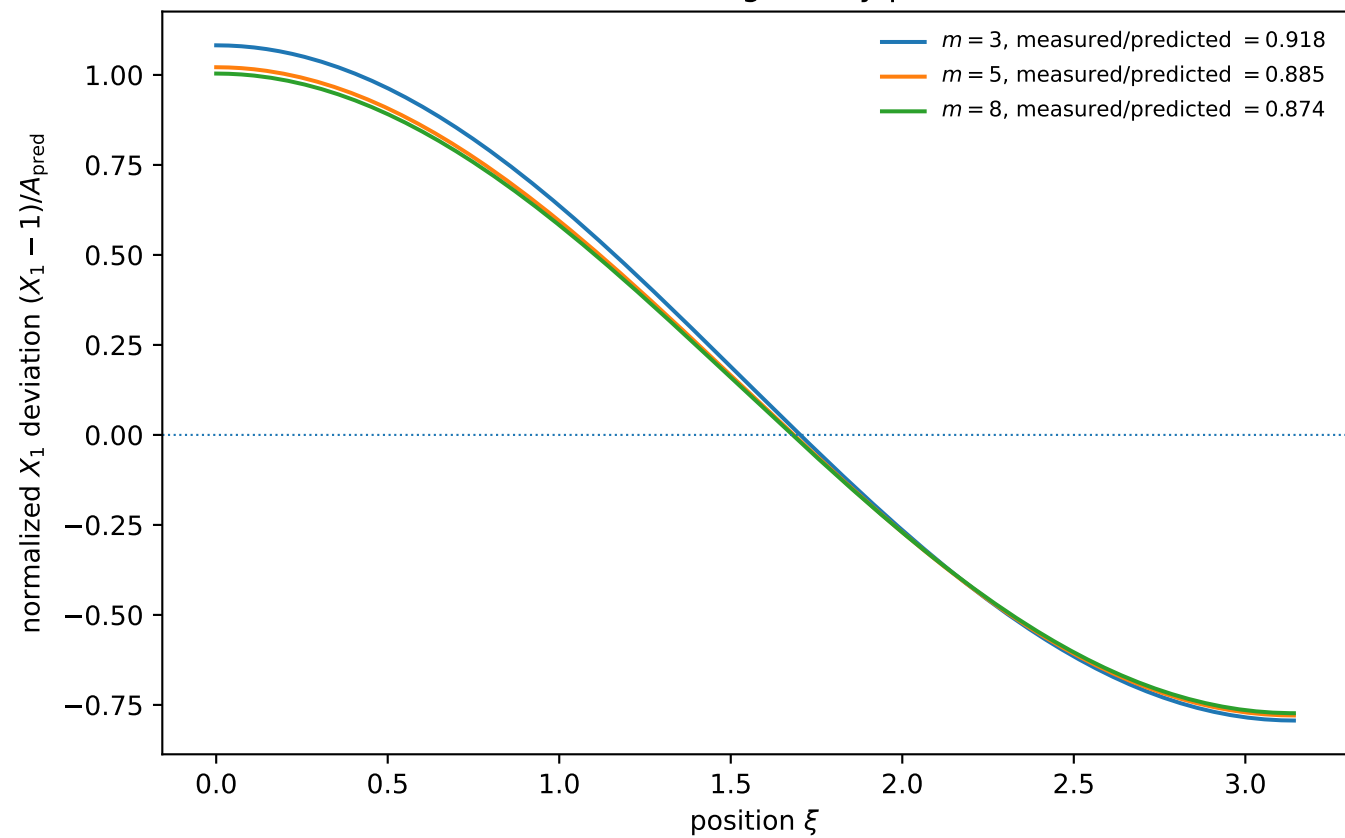
Numerical illustrations of the rigorously proved stable branches
