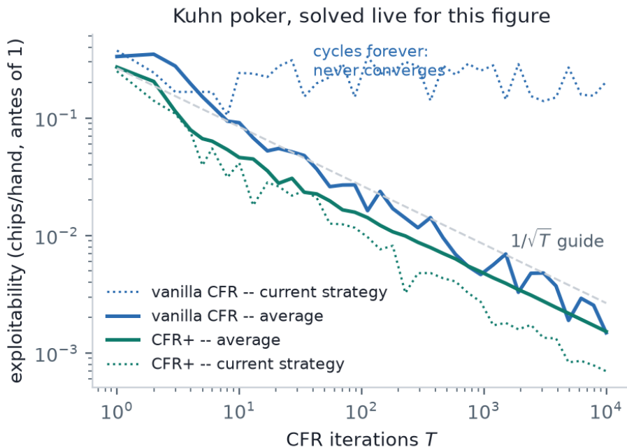
Figure 3: Real CFR runs on Kuhn poker (computed for this paper): average-strategy exploitability converges; current strategy either cycles (vanilla) or, under CFR+, converges on its own.
