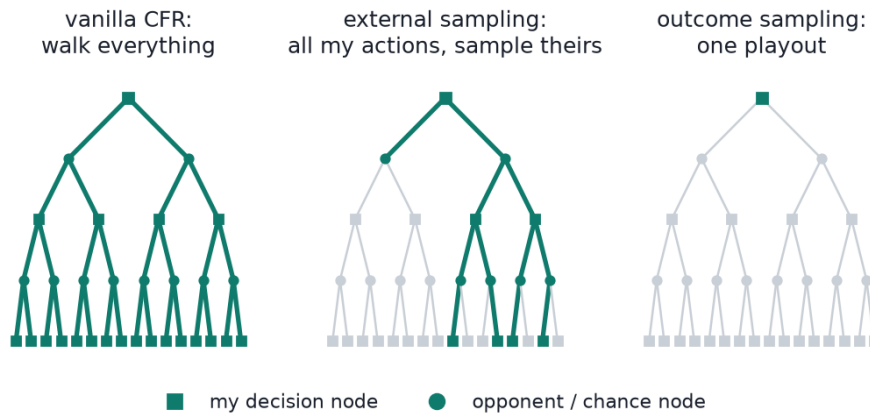
Figure 4: What one iteration touches under each traversal scheme (teal = visited).
