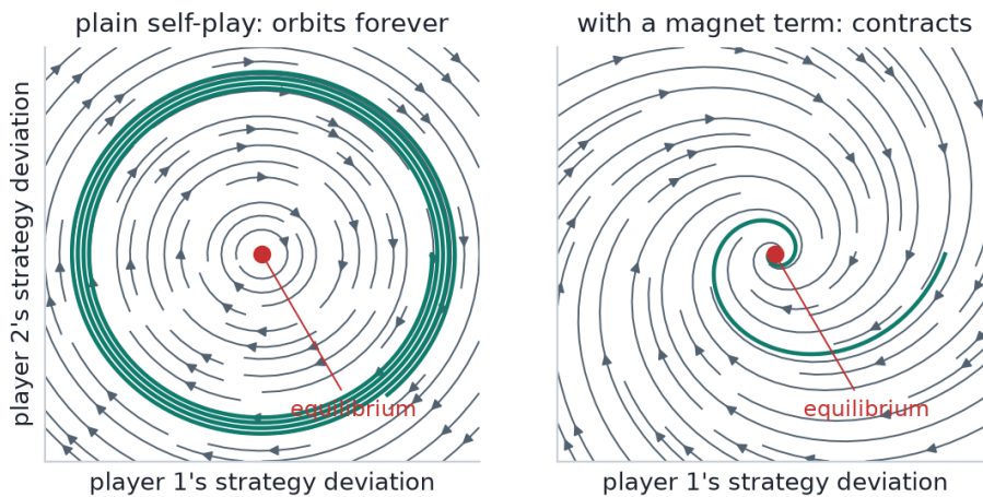
Figure 8: Real trajectories of the two dynamics (simulated for this paper): unregularized self-play orbits; adding a KL pull toward a reference policy makes the same dynamics contract.
