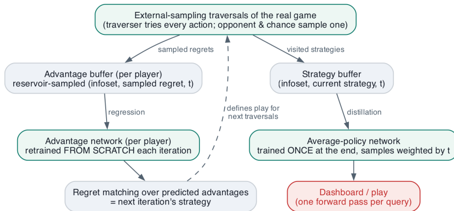
Figure 6: The Deep CFR training loop; teal = learned components, red = what the dashboard queries.
