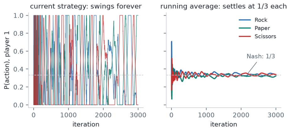
Figure 2: Both players running regret matching in rock-paper-scissors (simulated for this paper): current strategy vs. its running average.
