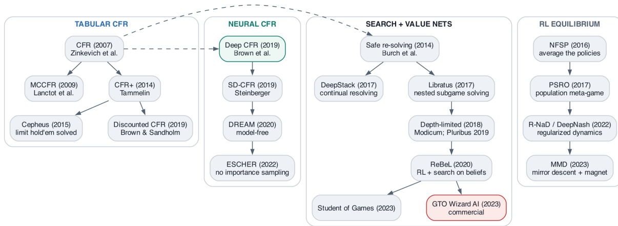
Figure 7: The four method families and their landmark systems; dashed arrows mark CFR’s ideas feeding the other lineages.
