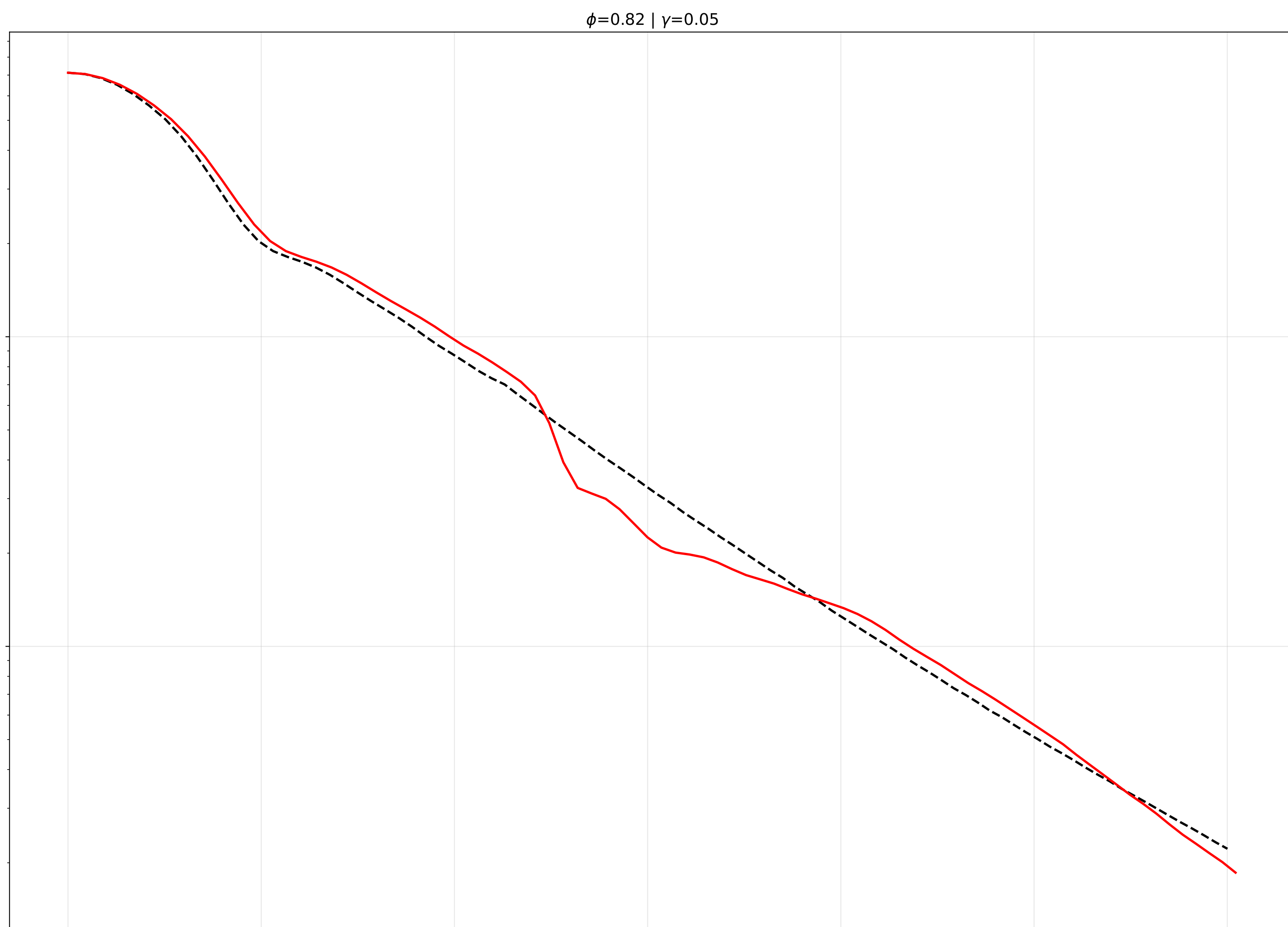
Async FIRE vs Global FIRE: 3x3 Short Sweep (N=100000)
