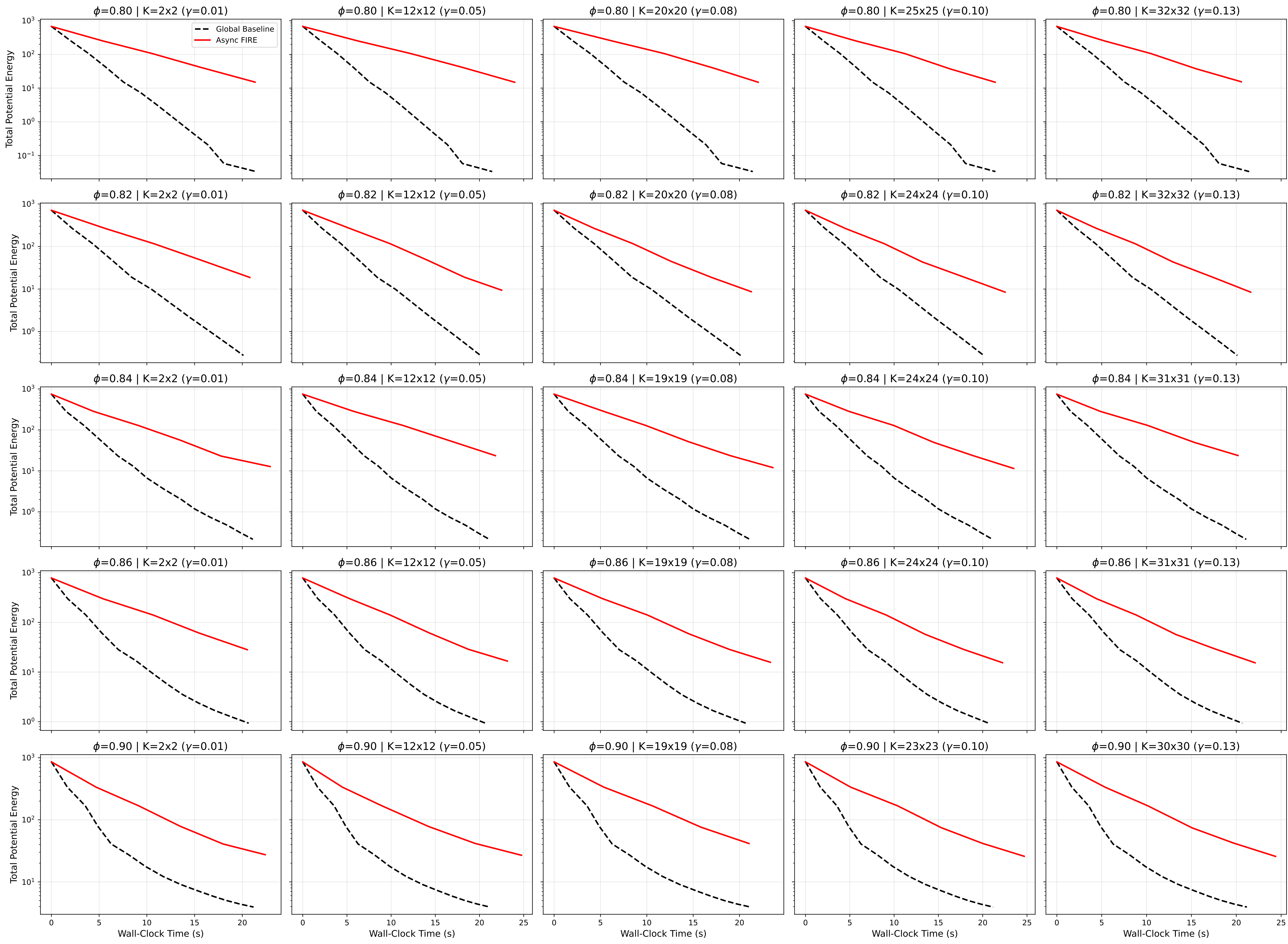
Async FIRE vs Global FIRE: Energy Convergence vs. Wall-Clock Time (N=1,000,000)
