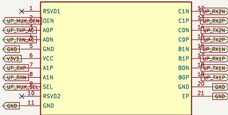
U1201 HD3SS3212IRKSR
