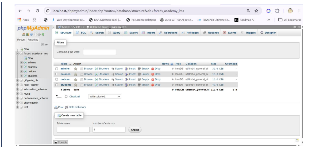
Fig. 1.1 — forces_academy_lms database structure, showing all four tables in phpMyAdmin
