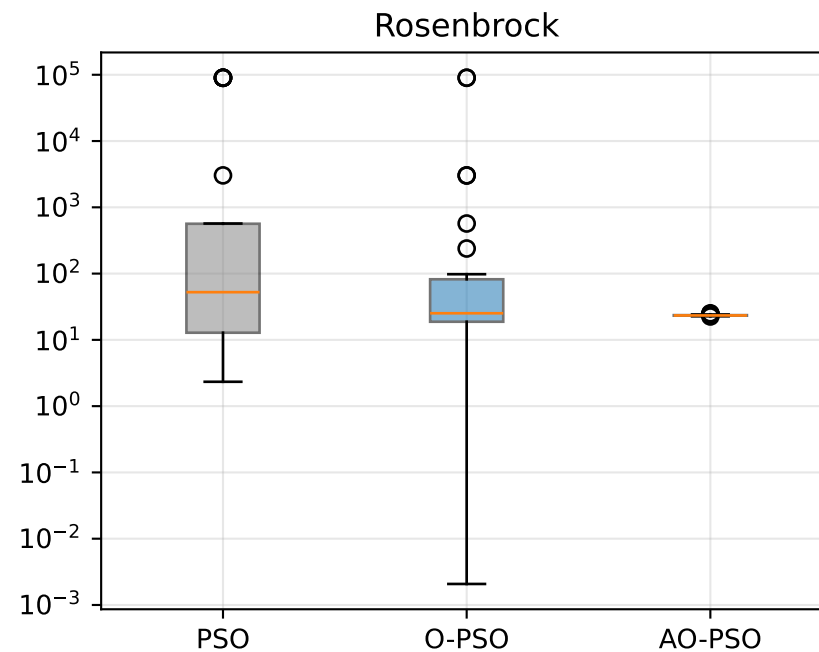
Final-fitness distribution at D=30 (30 runs)
