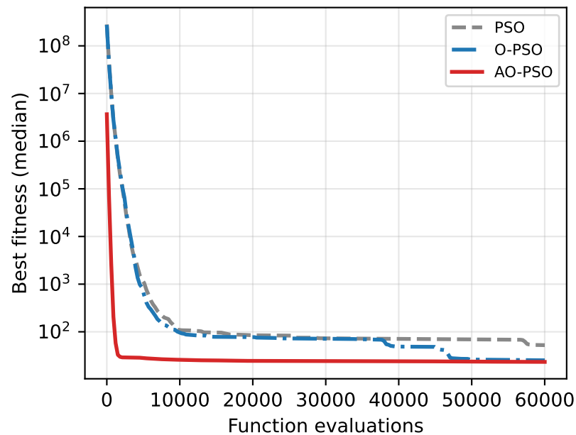
Ackley
