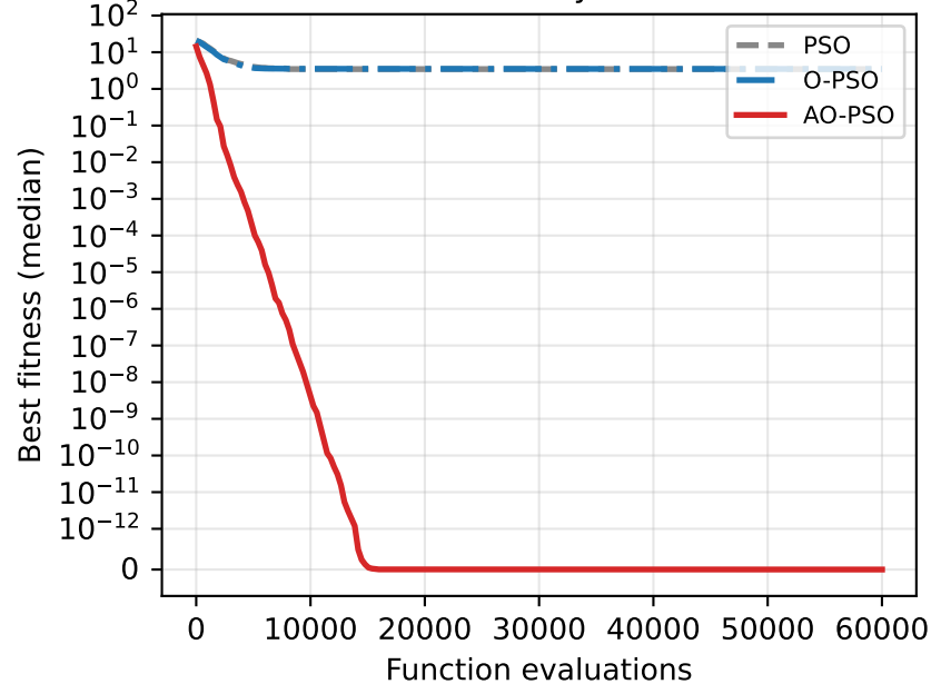
Ackley
